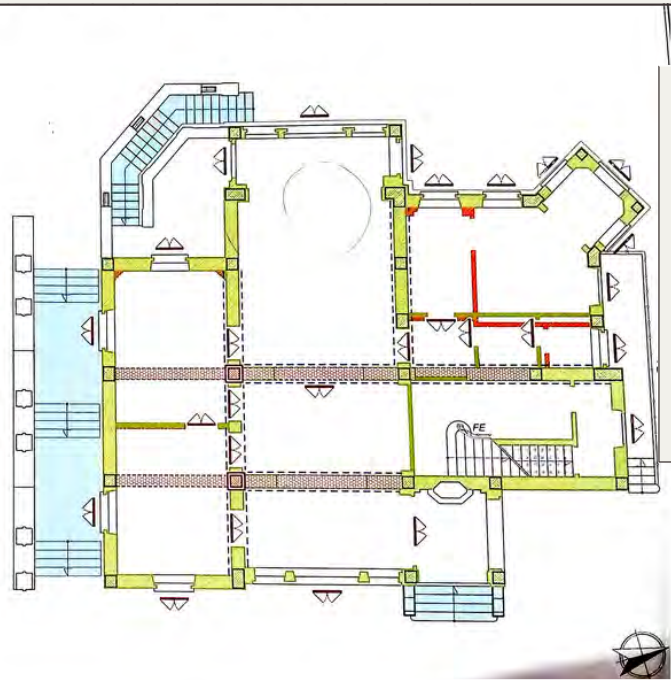
Piano terra
